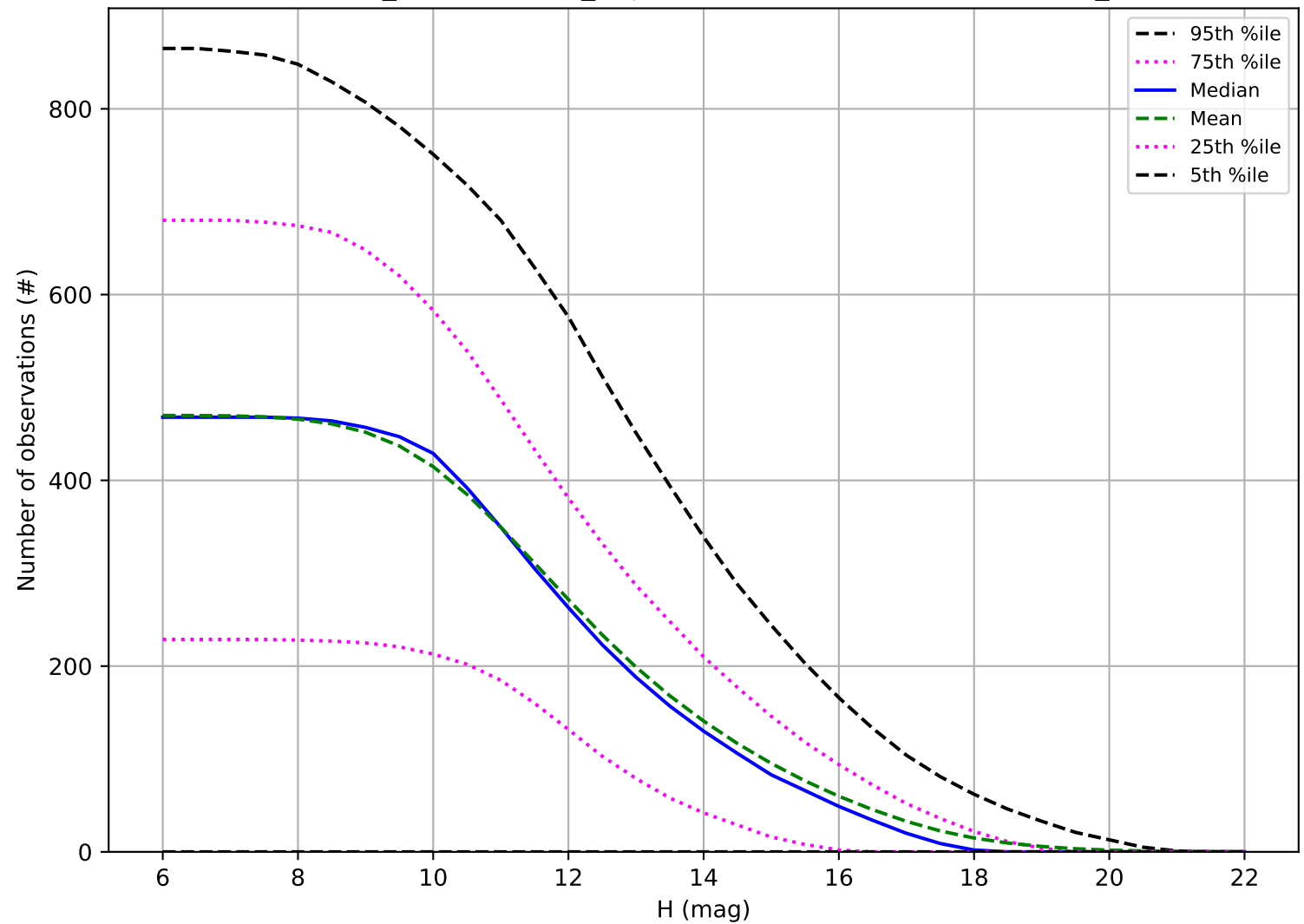
weather_cloudso1v3.4_10yrs: Number of observations OCC_r5
