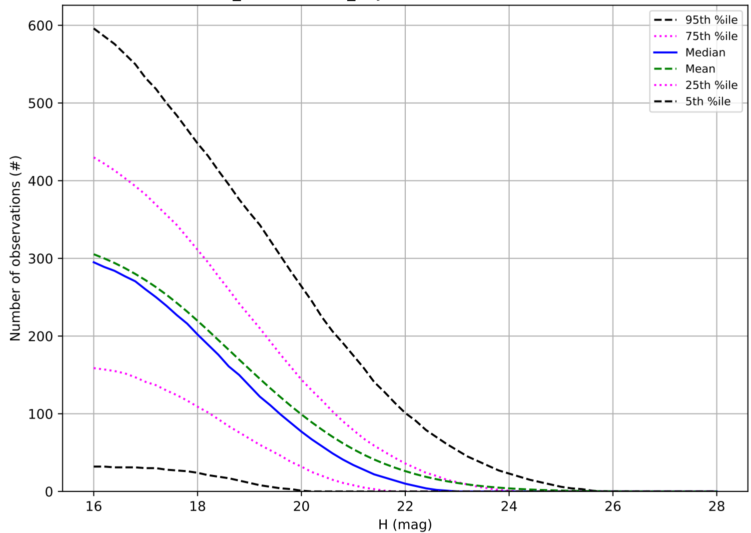
weather_cloudso1v3.4_10yrs: Number of observations NEO
