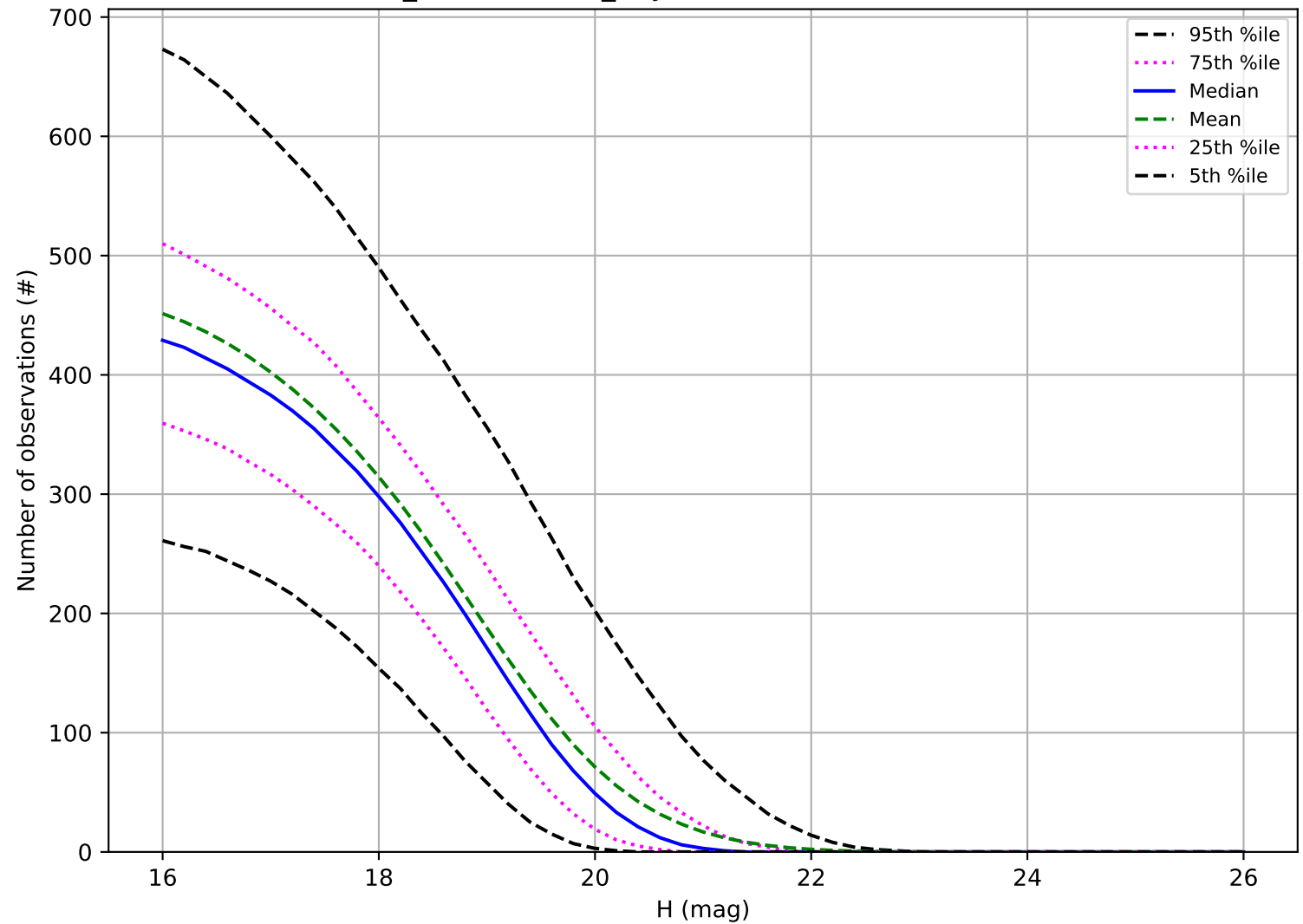
weather_cloudso1v3.4_10yrs: Number of observations MBA
