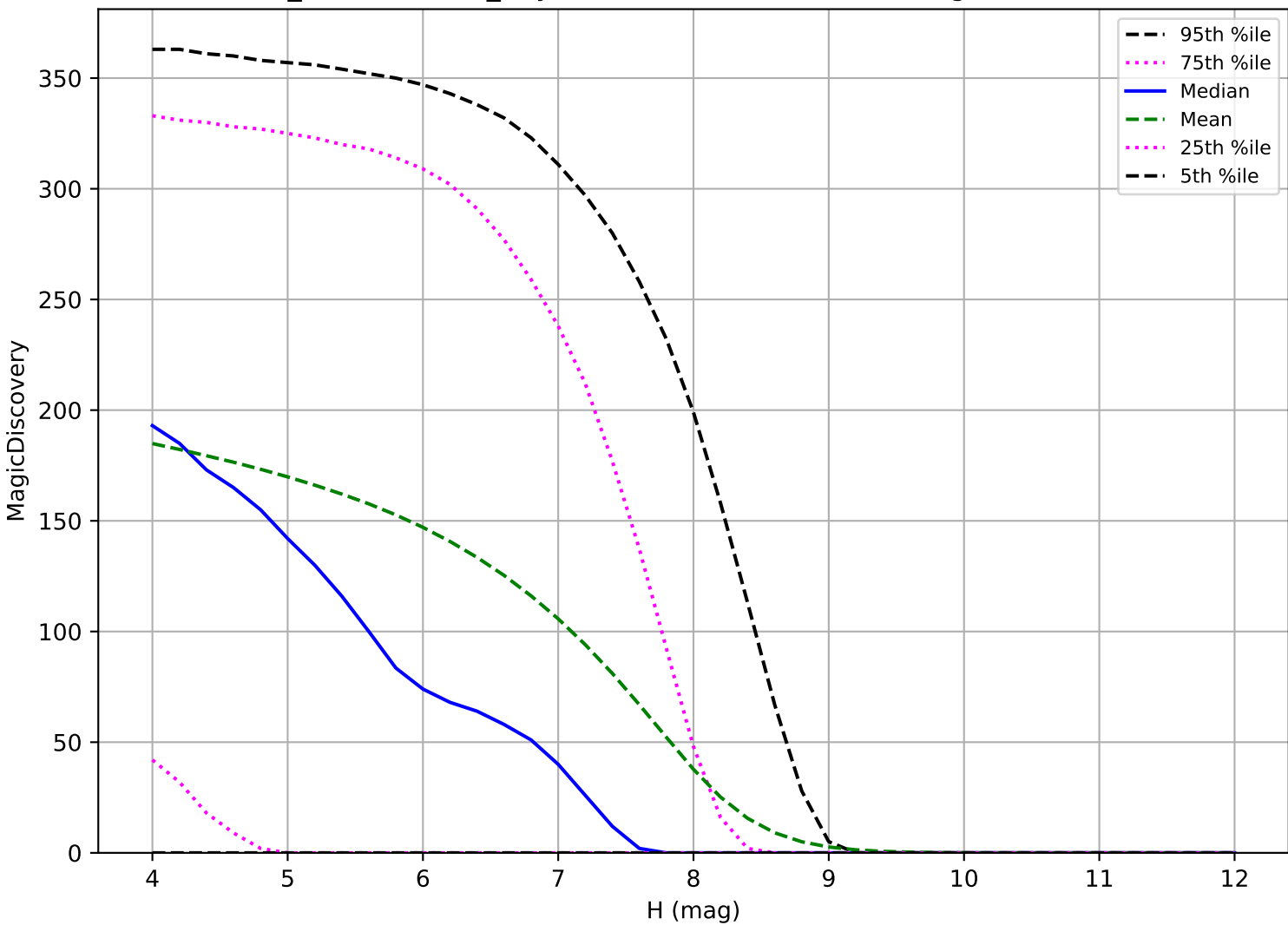
weather_cloudso1v3.4_10yrs: TNO 6 detections in 60 nights detection loss
