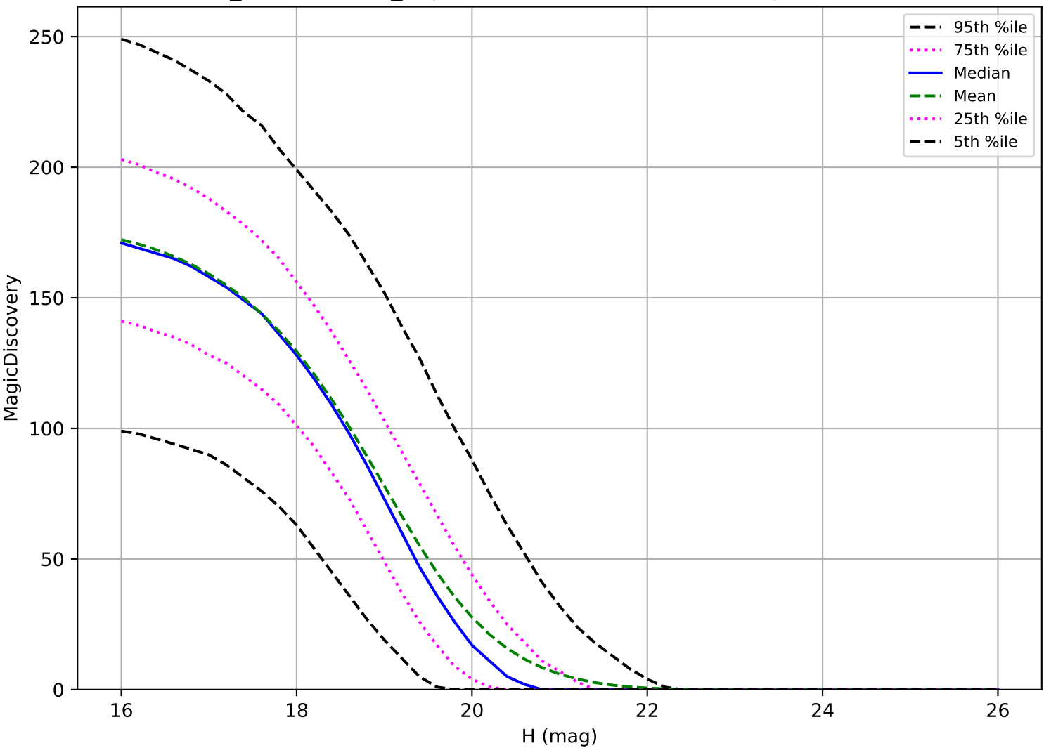
weather_cloudso1v3.4_10yrs: MBA 6 detections in 60 nights detection loss
