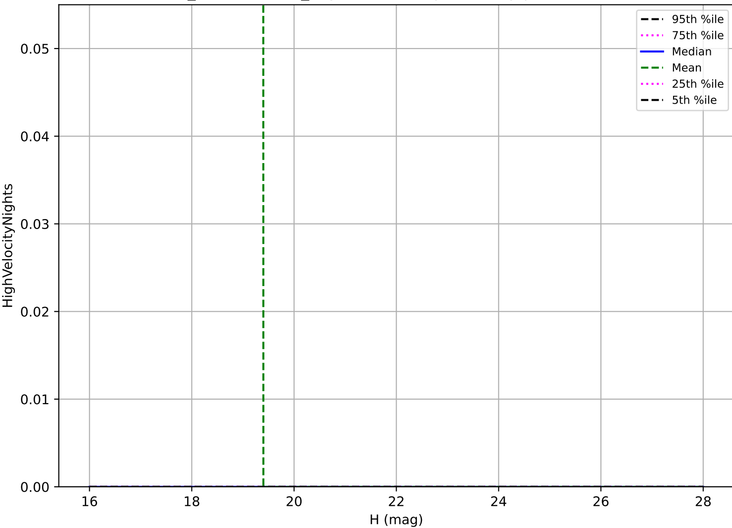
weather_cloudso1v3.4_10yrs: Vatira High velocity pair detection loss
