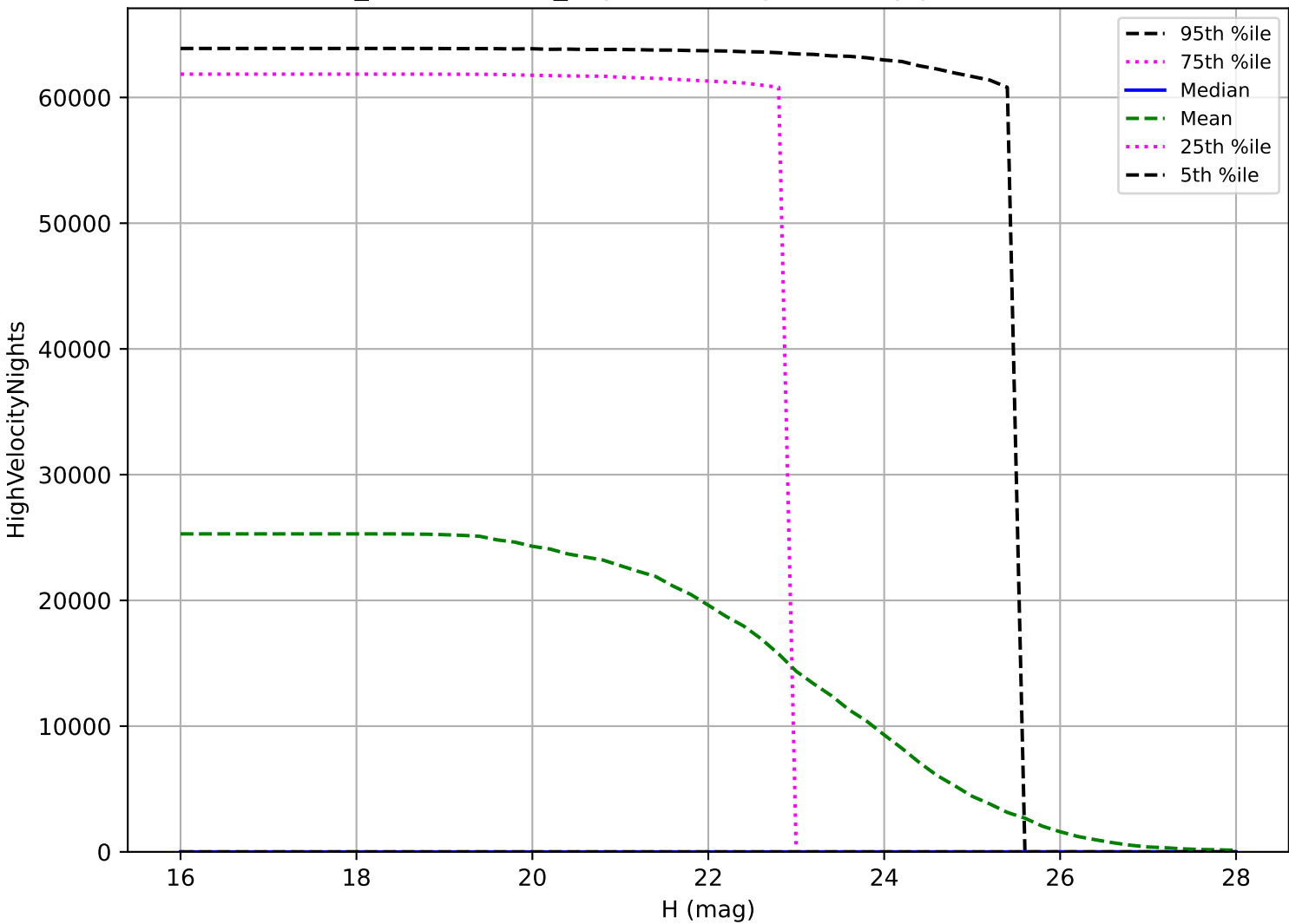
weather_cloudso1v3.4_10yrs: PHA High velocity pair detection loss
