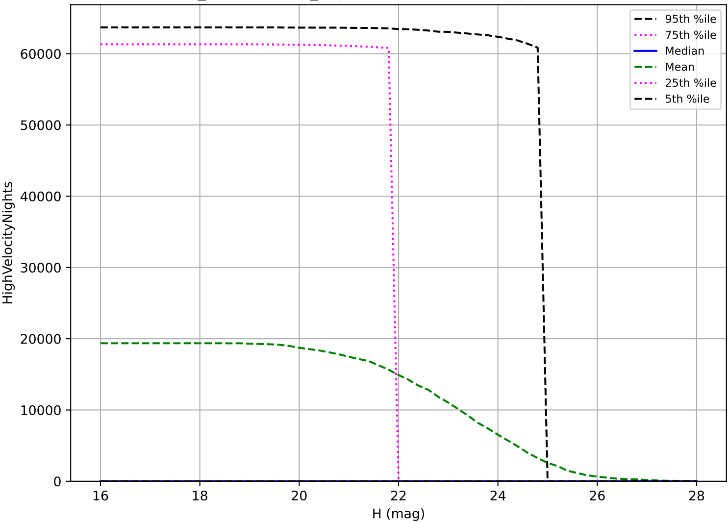
weather_cloudso1v3.4_10yrs: NEO High velocity pair detection loss
