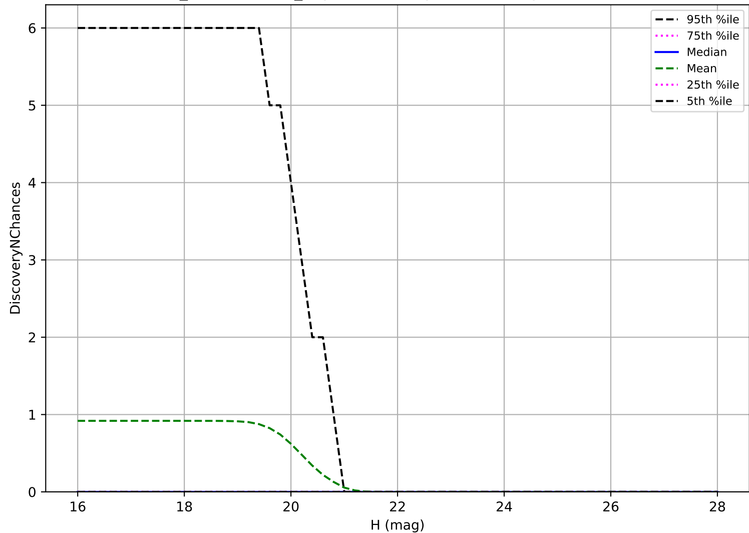
weather_cloudso1v3.4_10yrs: Vatira 3 pairs in 15 nights detection loss
