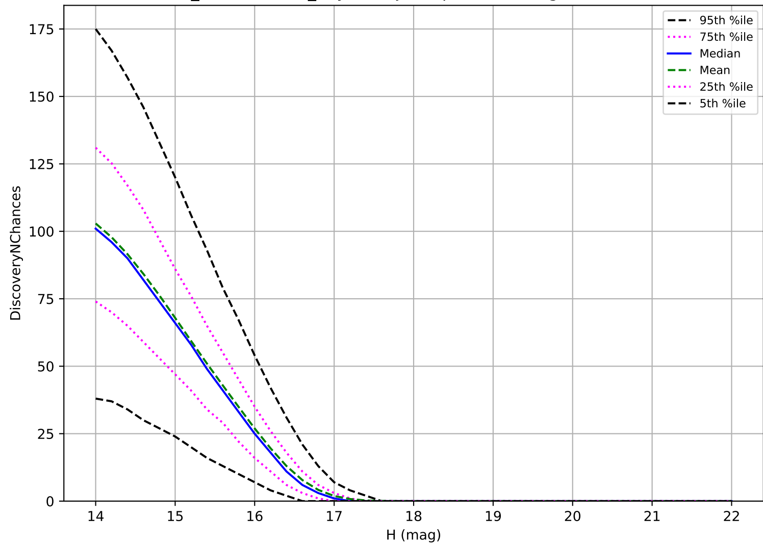
weather_cloudso1v3.4_10yrs: Trojan 3 pairs in 15 nights detection loss
