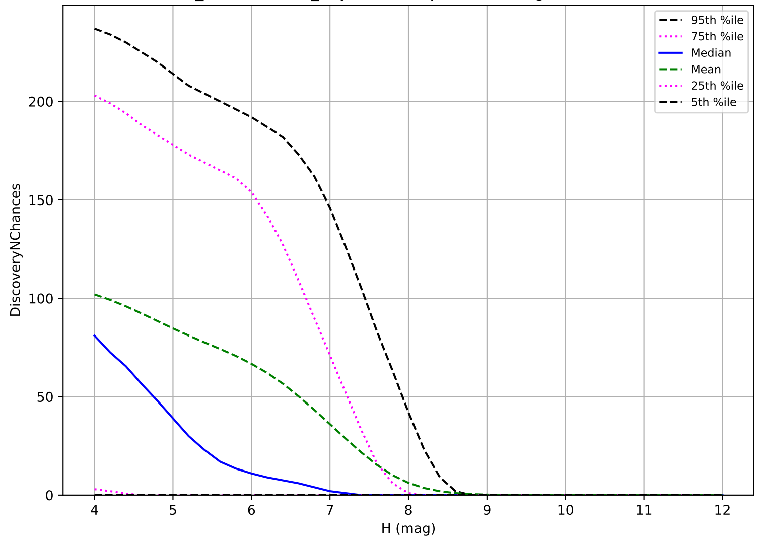
weather_cloudso1v3.4_10yrs: TNO 3 pairs in 15 nights detection loss
