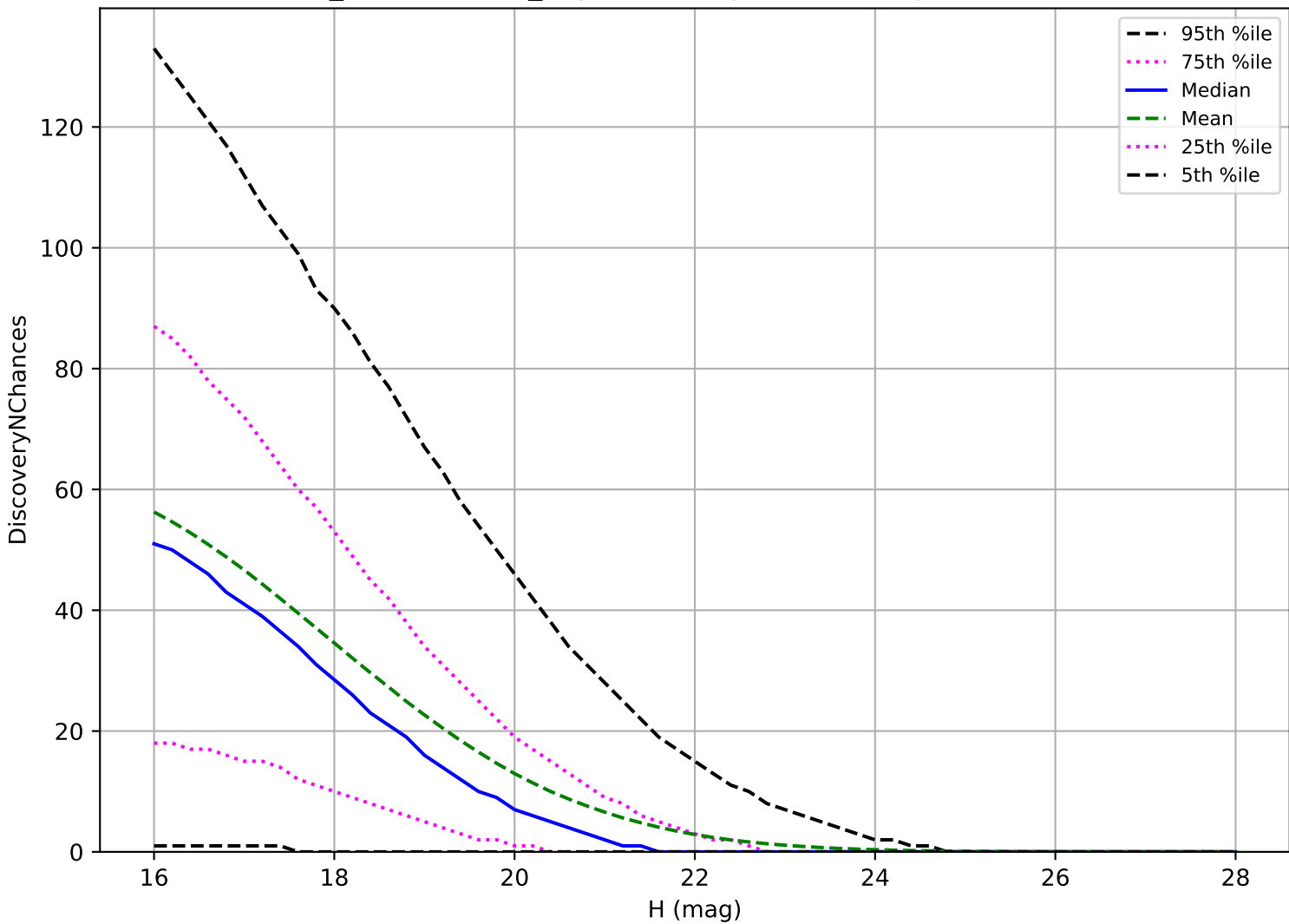
weather_cloudso1v3.4_10yrs: PHA 3 pairs in 15 nights detection loss
