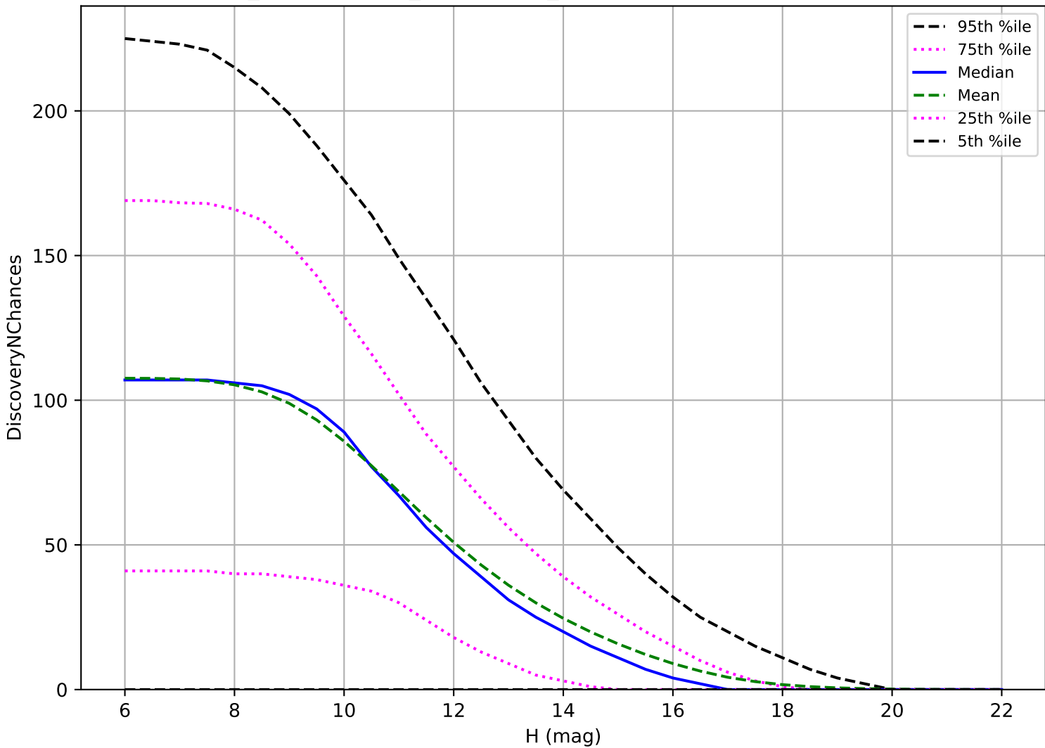
weather_cloudso1v3.4_10yrs: OCC_r5 3 pairs in 15 nights detection loss
