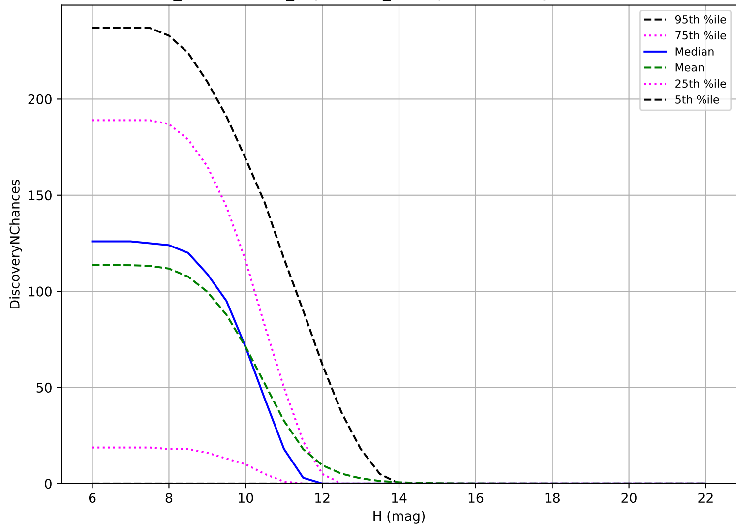
weather_cloudso1v3.4_10yrs: OCC_r20 3 pairs in 15 nights detection loss
