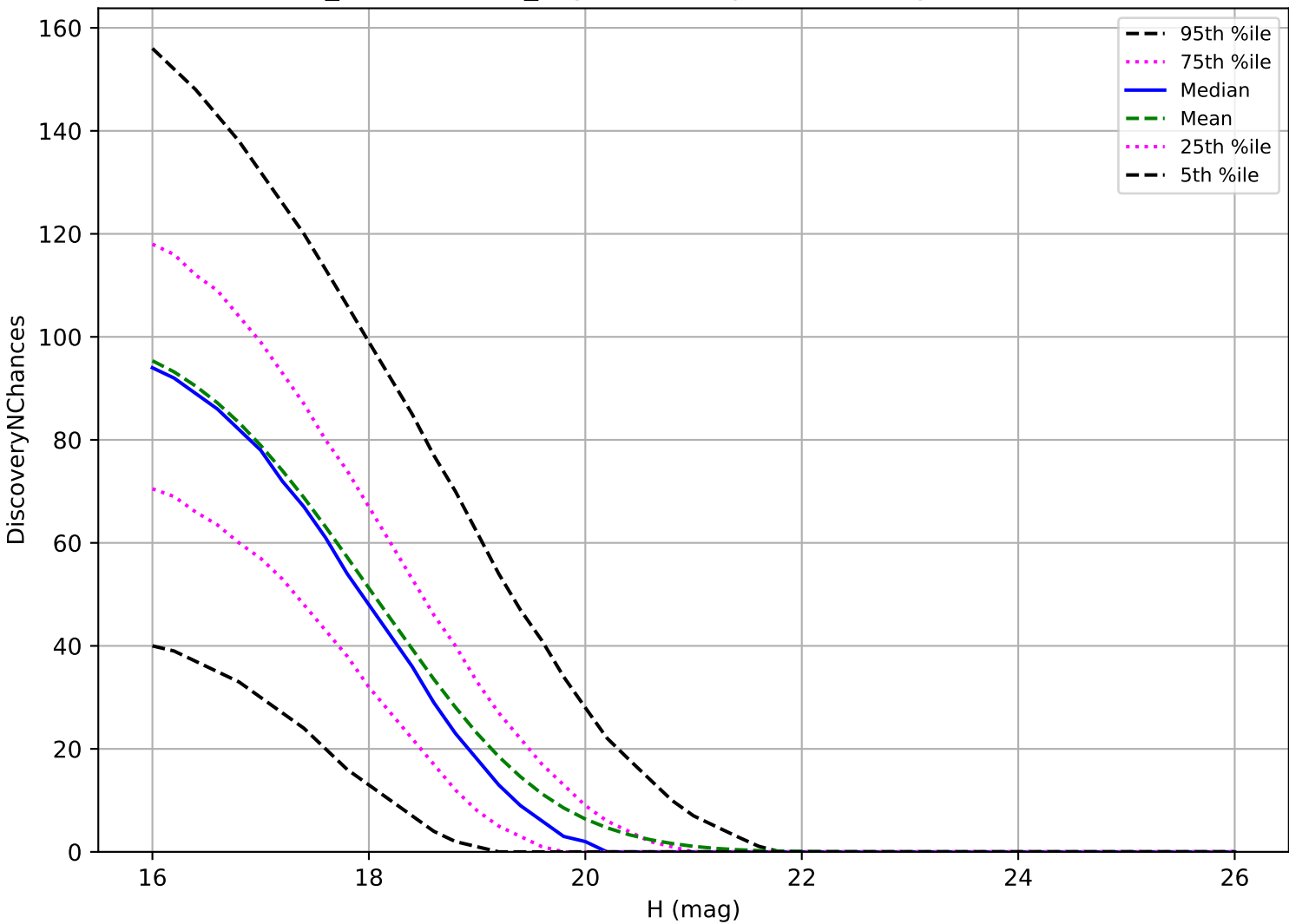
weather_cloudso1v3.4_10yrs: MBA 3 pairs in 15 nights detection loss
