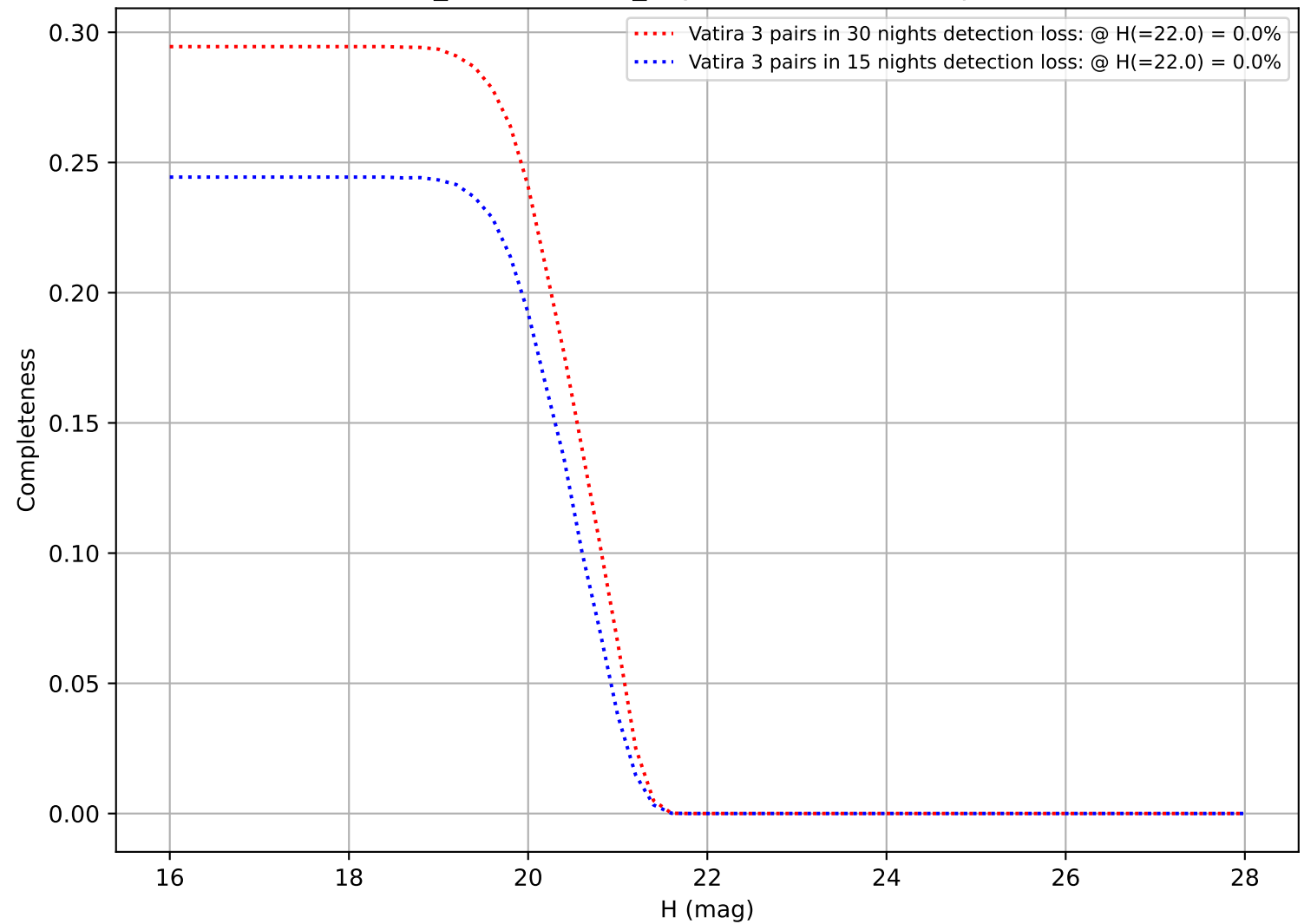
weather_cloudso1v3.4_10yrs: DifferentialCompleteness
