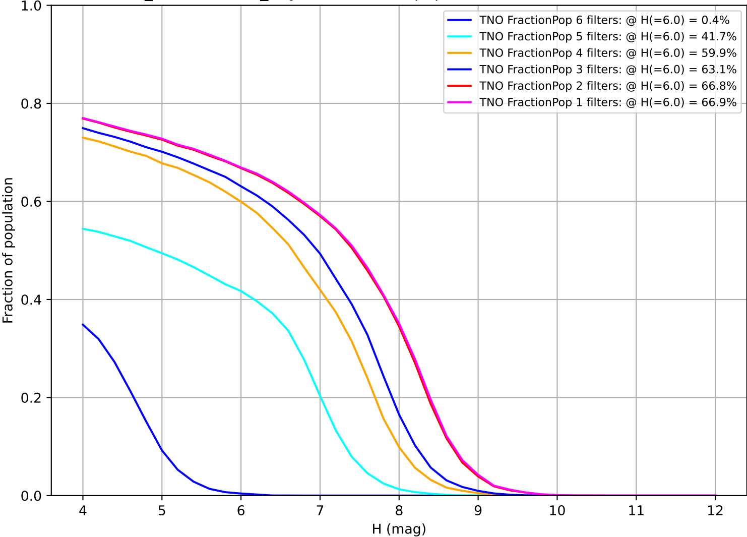
weather_cloudso1v3.4_10yrs: Fraction of population with colors in X filters TNO
