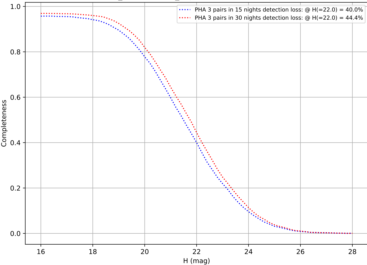
weather_cloudso1v3.4_10yrs: DifferentialCompleteness
