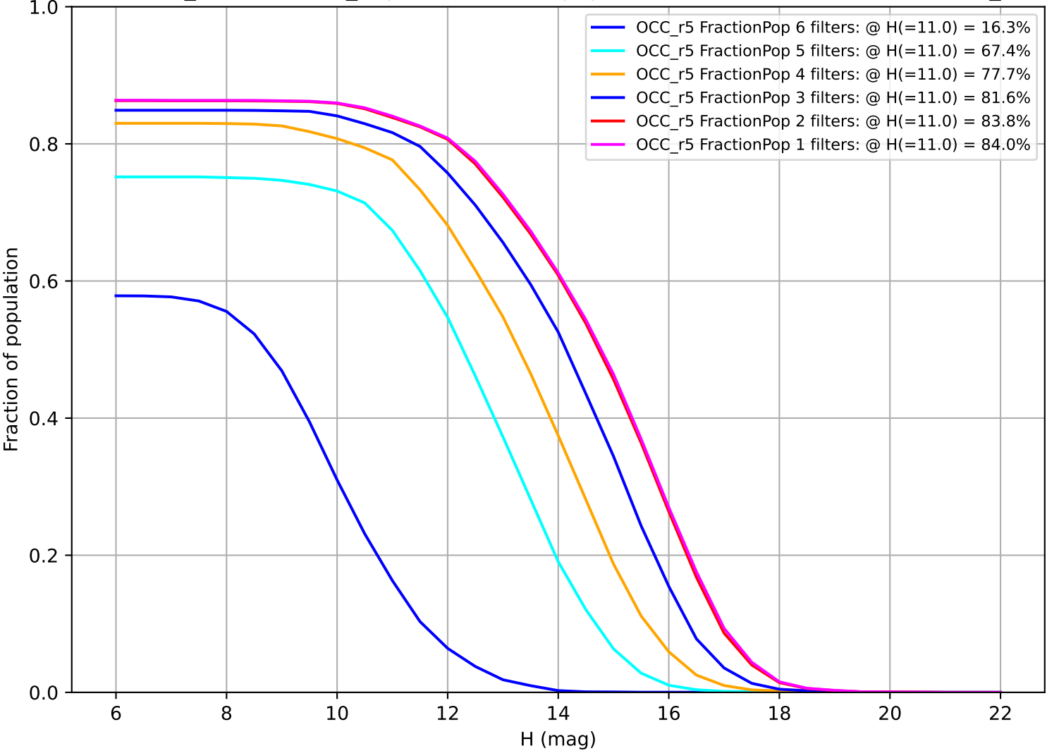
weather_cloudso1v3.4_10yrs: Fraction of population with colors in X filters OCC_r5
