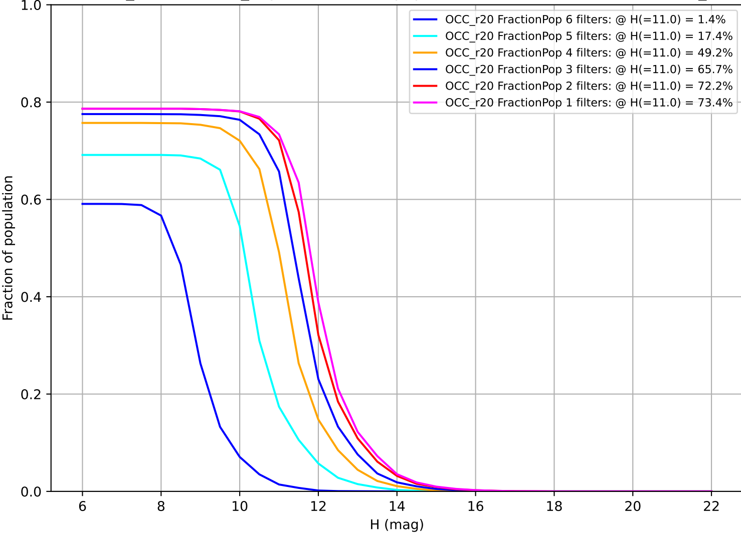
weather_cloudso1v3.4_10yrs: Fraction of population with colors in X filters OCC_r20
