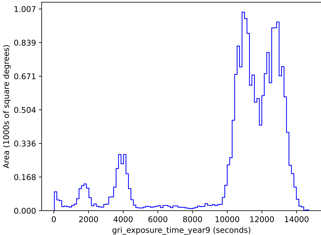
weather_cloudso1v3.4_10yrs gri band non-DD: gri_exposure_time_year9
