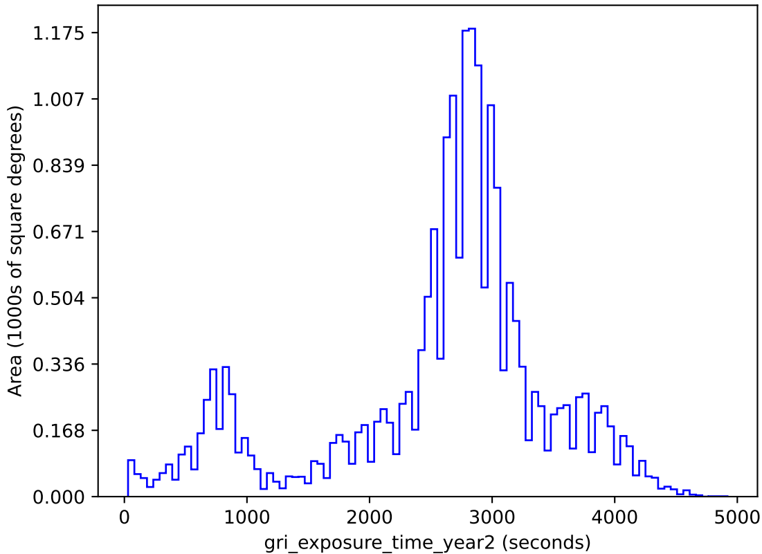
weather_cloudso1v3.4_10yrs gri band non-DD: gri_exposure_time_year2
