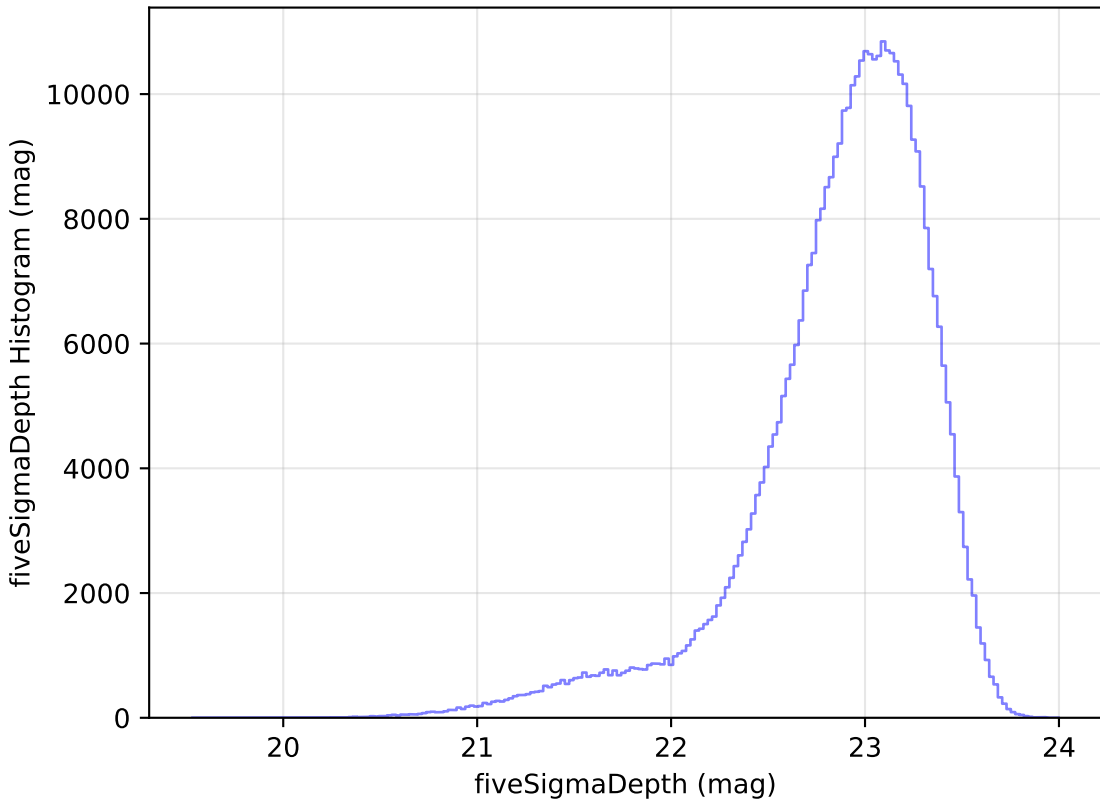
weather_cloudso1v3.4_10yrs z: fiveSigmaDepth Histogram
