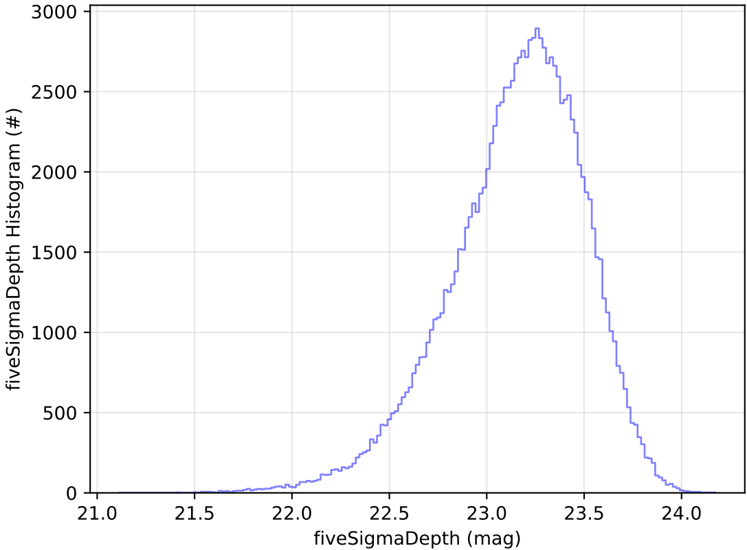
weather_cloudso1v3.4_10yrs u: fiveSigmaDepth Histogram
