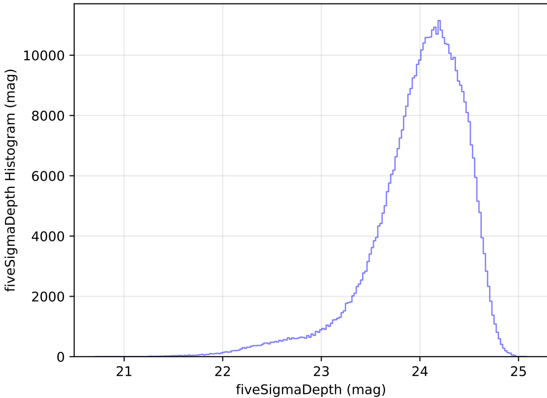
weather_cloudso1v3.4_10yrs r: fiveSigmaDepth Histogram
