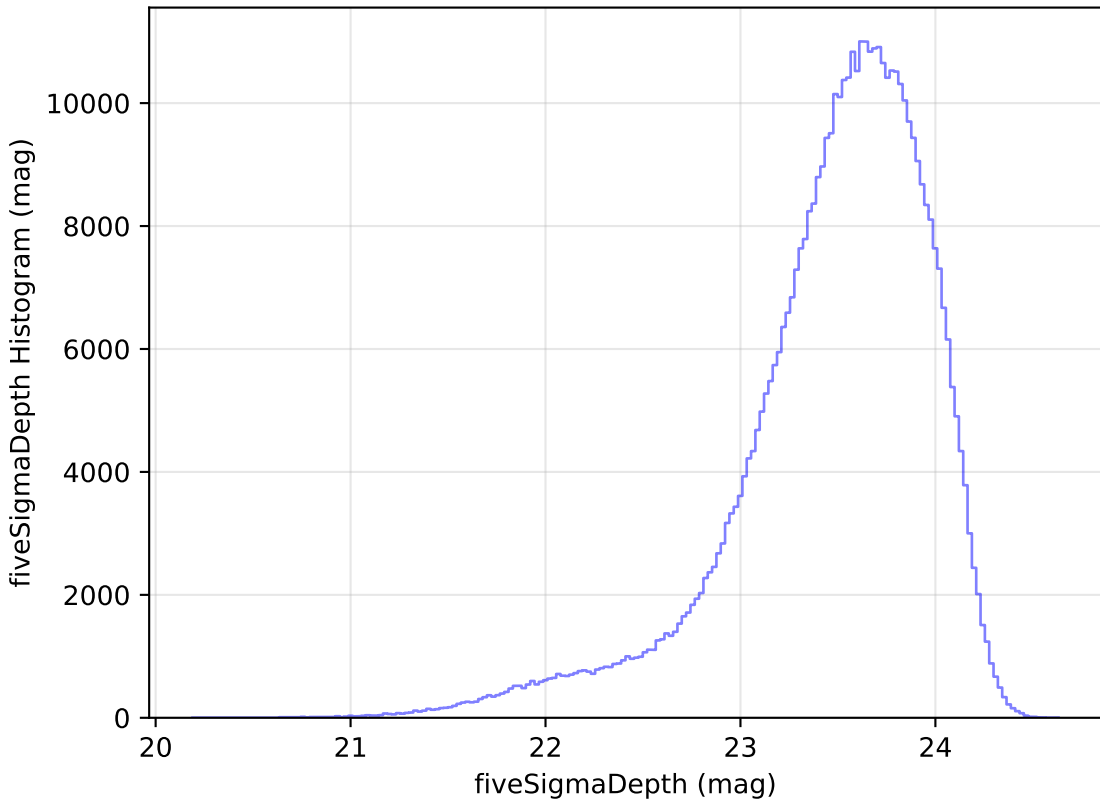
weather_cloudso1v3.4_10yrs i: fiveSigmaDepth Histogram
