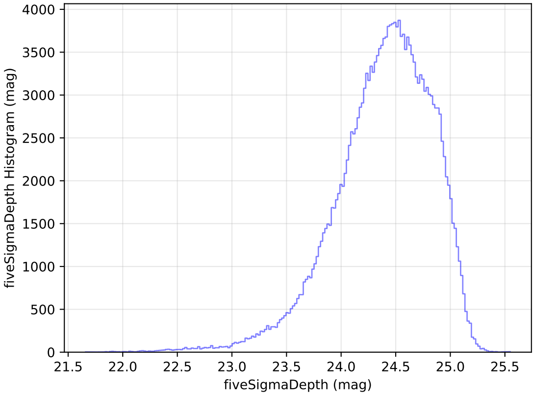
weather_cloudso1v3.4_10yrs g: fiveSigmaDepth Histogram
