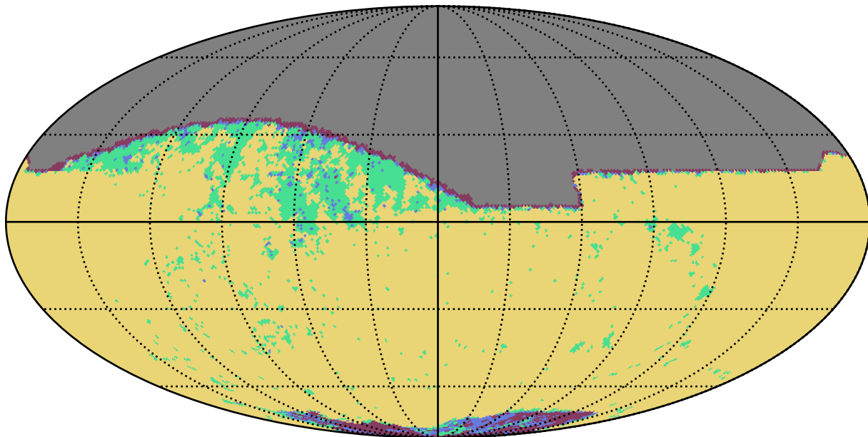
weather_cloudso1v3.4_10yrs z band: YearCoverage night
