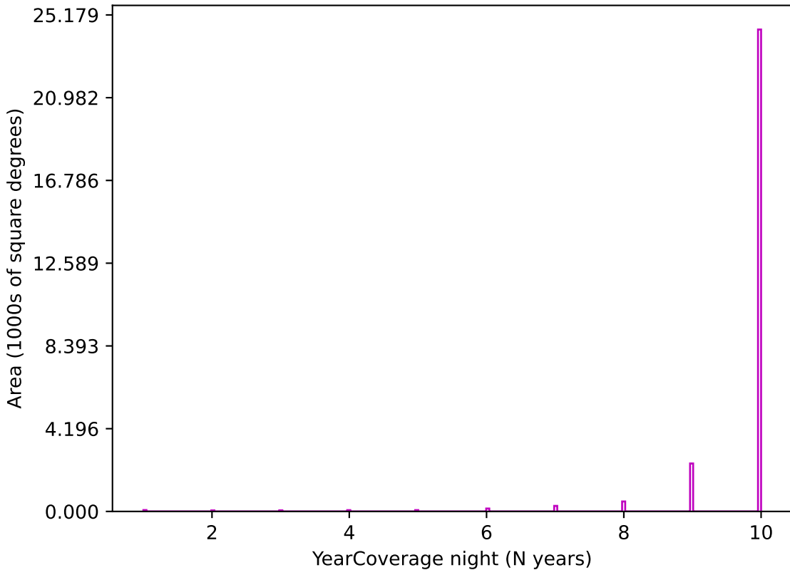
weather_cloudso1v3.4_10yrs z band: YearCoverage night
