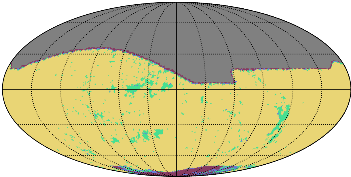
weather_cloudso1v3.4_10yrs r band: YearCoverage night
