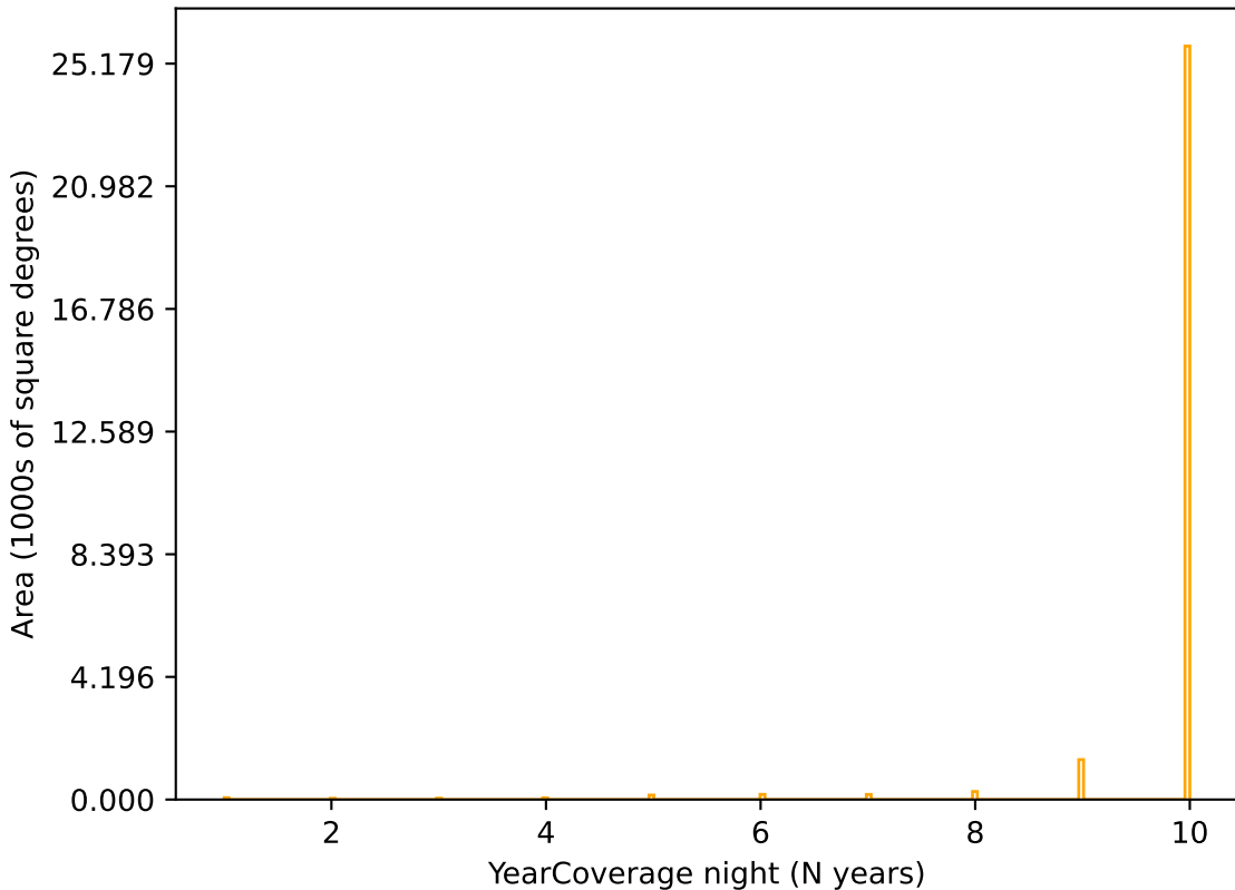
weather_cloudso1v3.4_10yrs r band: YearCoverage night
