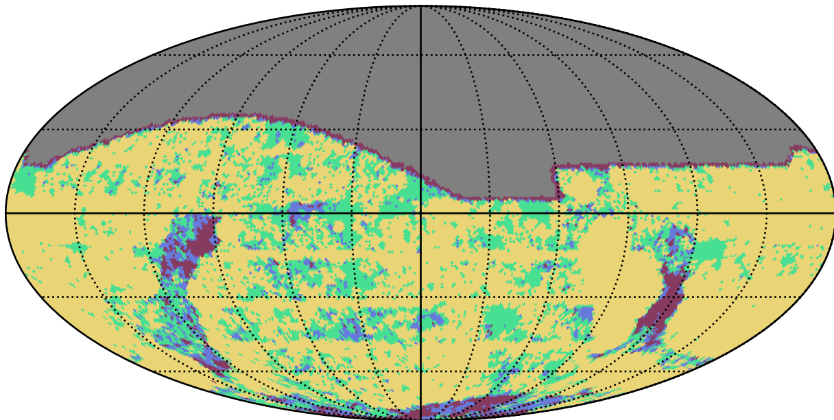
weather_cloudso1v3.4_10yrs g band: YearCoverage night
