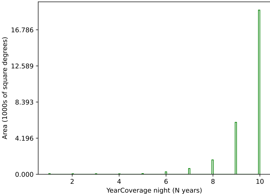
weather_cloudso1v3.4_10yrs g band: YearCoverage night
