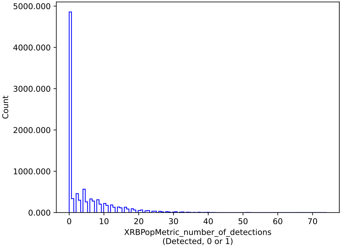
weather_cloudso1v3.4_10yrs : XRBPoMetric_number_of_detections
