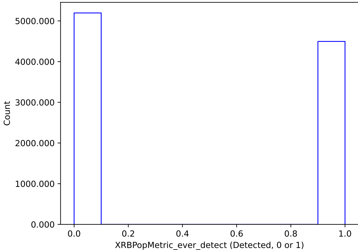
weather_cloudso1v3.4_10yrs : XRBPoMetric_ever_detect
