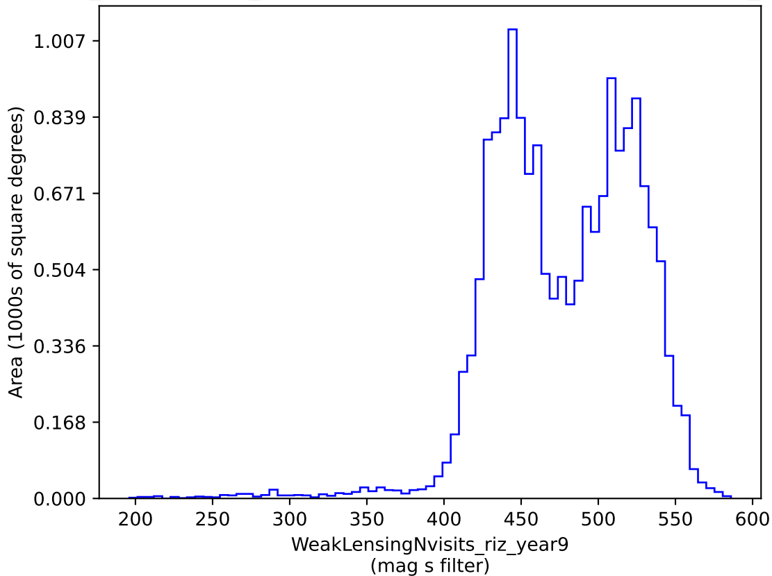
weather_cloudso1v3.4_10yrs gri band non-DD: WeakLensingNvisits_riz_year9
