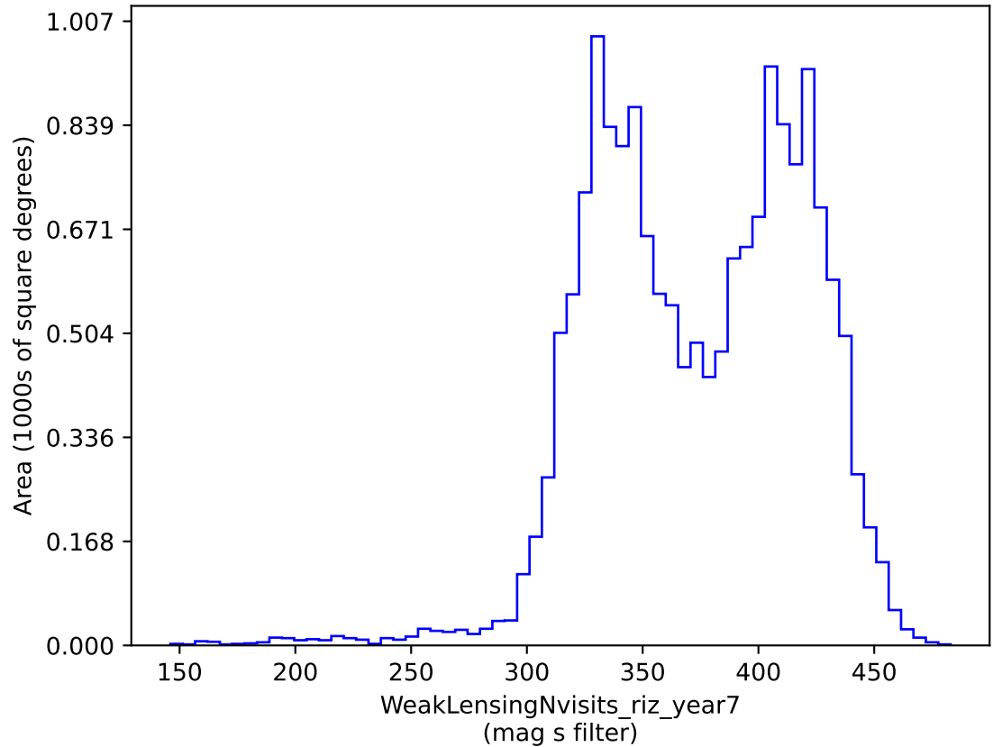
weather_cloudso1v3.4_10yrs gri band non-DD: WeakLensingNvisits_riz_year7
