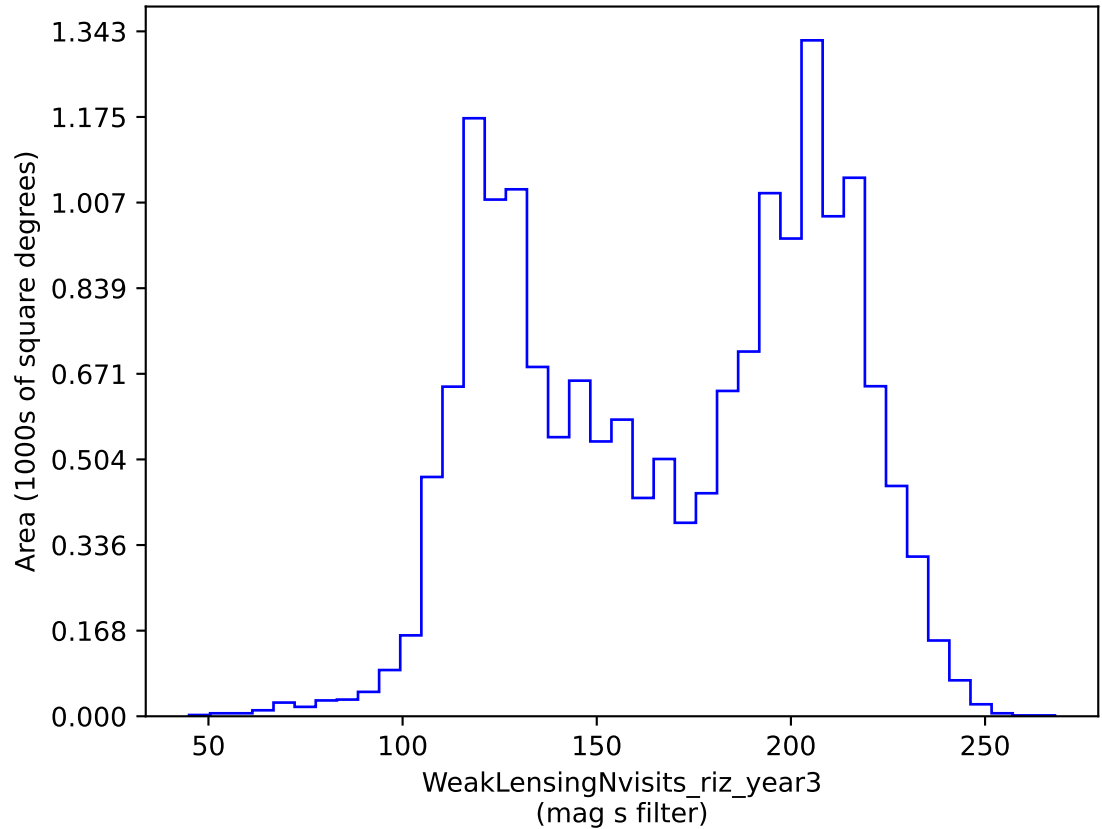
weather_cloudso1v3.4_10yrs gri band non-DD: WeakLensingNvisits_riz_year3
