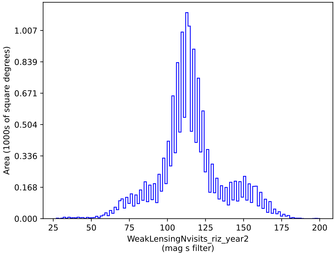
weather_cloudso1v3.4_10yrs gri band non-DD: WeakLensingNvisits_riz_year2
