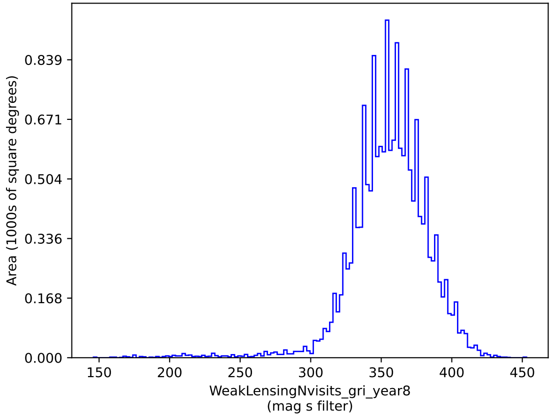
weather_cloudso1v3.4_10yrs gri band non-DD: WeakLensingNvisits_gri_year8
