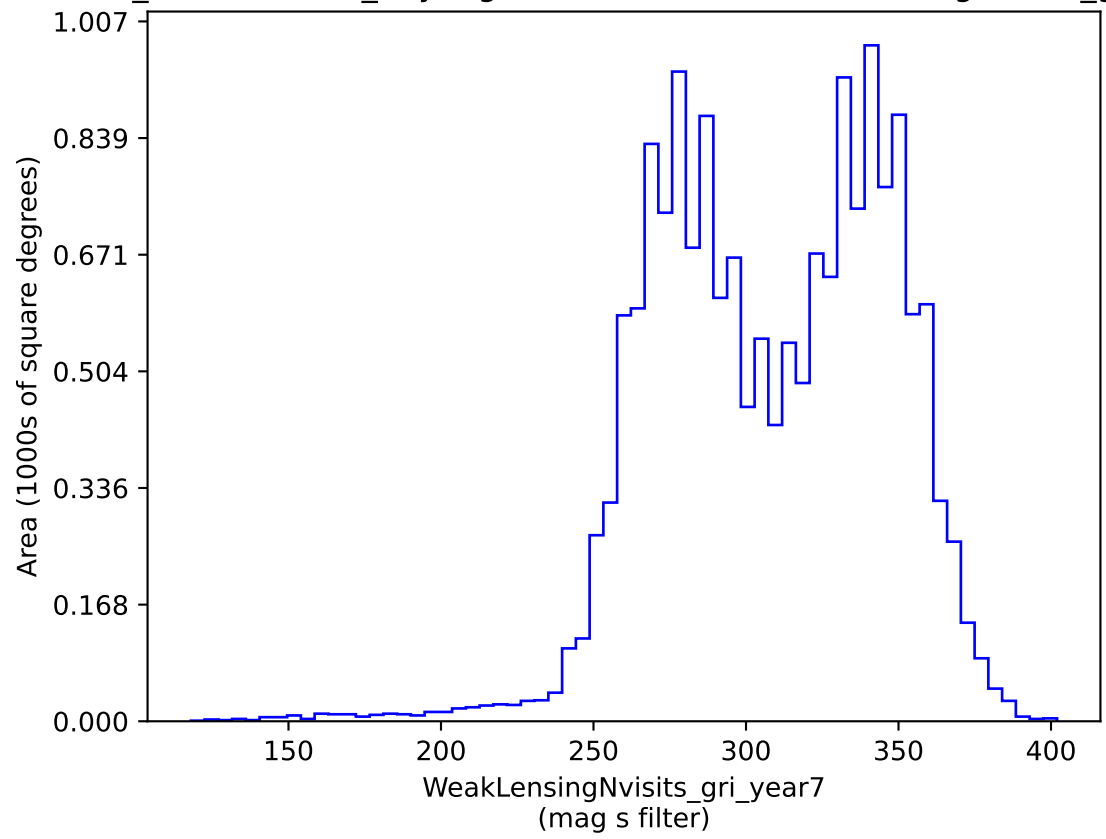
weather_cloudso1v3.4_10yrs gri band non-DD: WeakLensingNvisits_gri_year7
