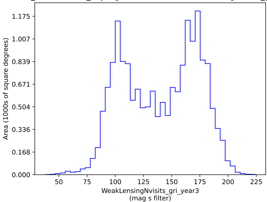
weather_cloudso1v3.4_10yrs gri band non-DD: WeakLensingNvisits_gri_year3
