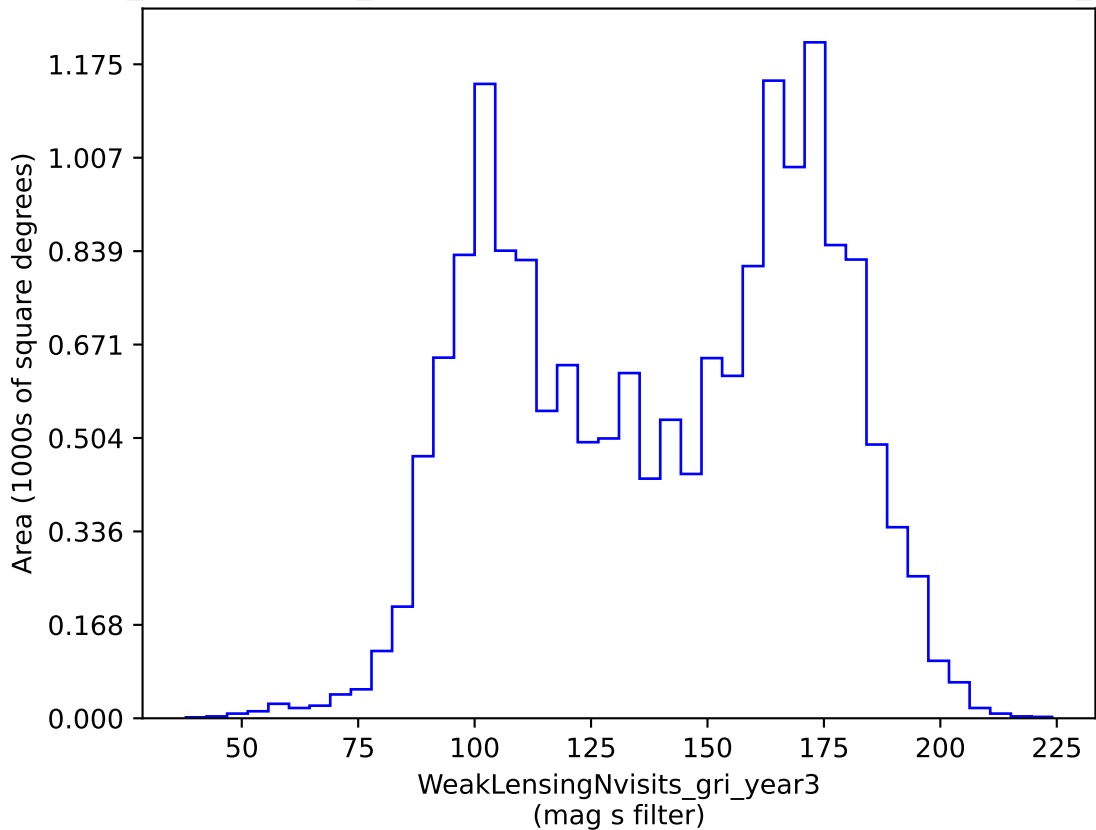
weather_cloudso1v3.4_10yrs gri band non-DD: WeakLensingNvisits_gri_year3
