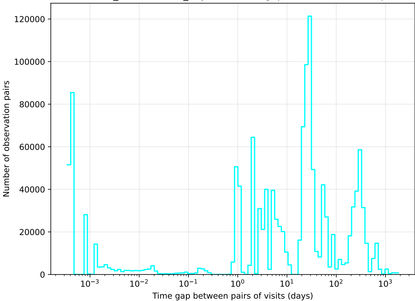
weather_cloudso1v3.4_10yrs u band: Tgaps observationStartMJD
