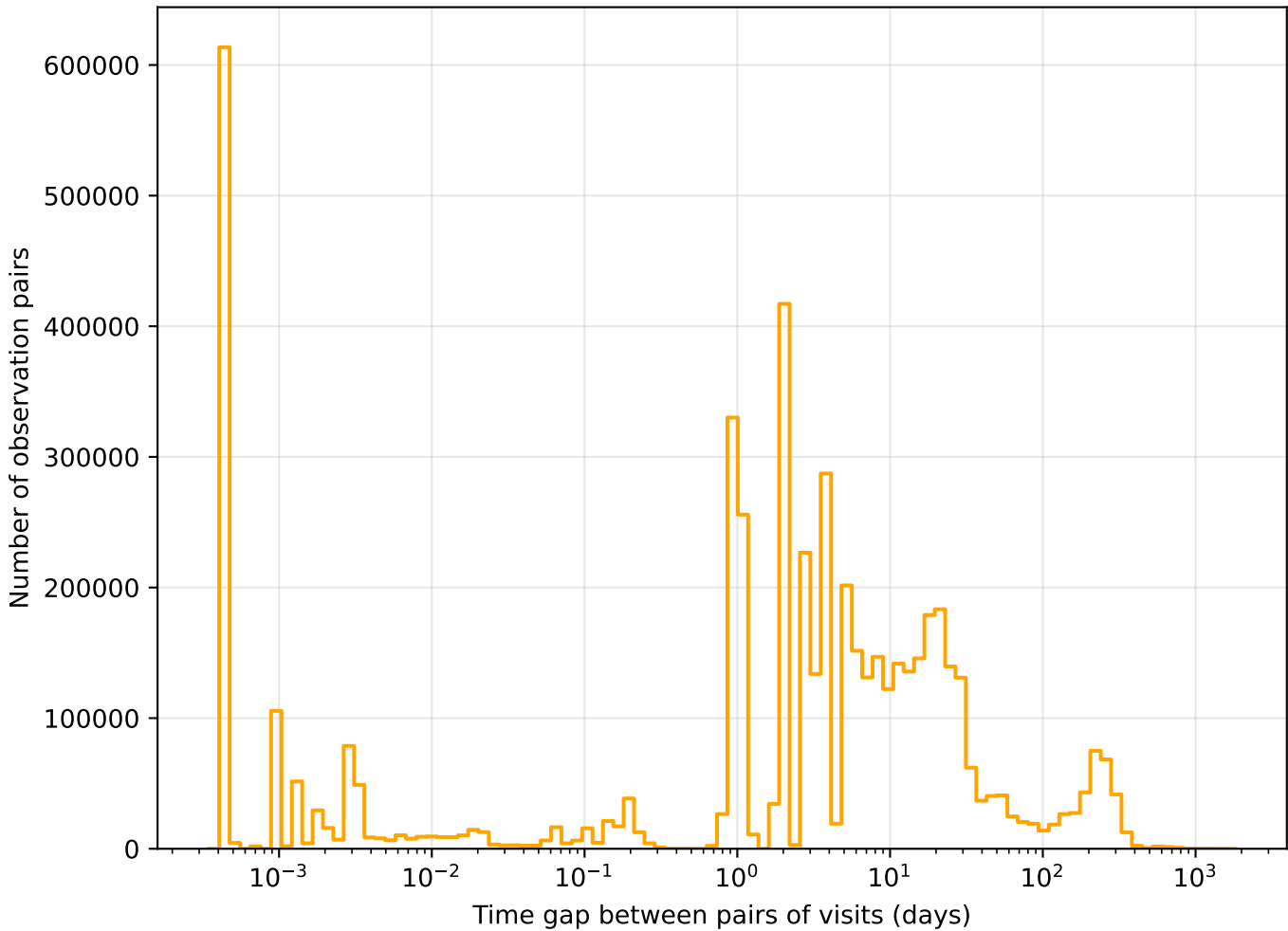
weather_cloudso1v3.4_10yrs r band: Tgaps observationStartMJD
