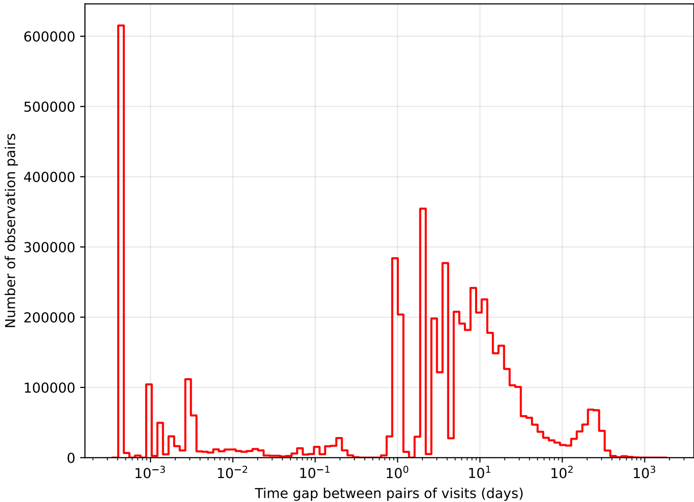
weather_cloudso1v3.4_10yrs i band: Tgaps observationStartMJD
