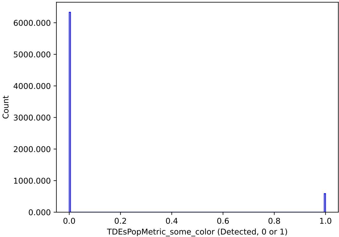
weather_cloudso1v3.4_10yrs : TDEsPopMetric_some_color
