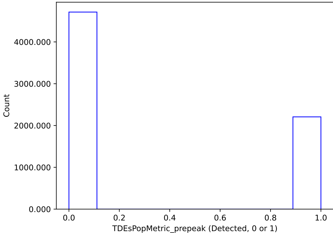
weather_cloudso1v3.4_10yrs : TDEsPopMetric_prepeak
