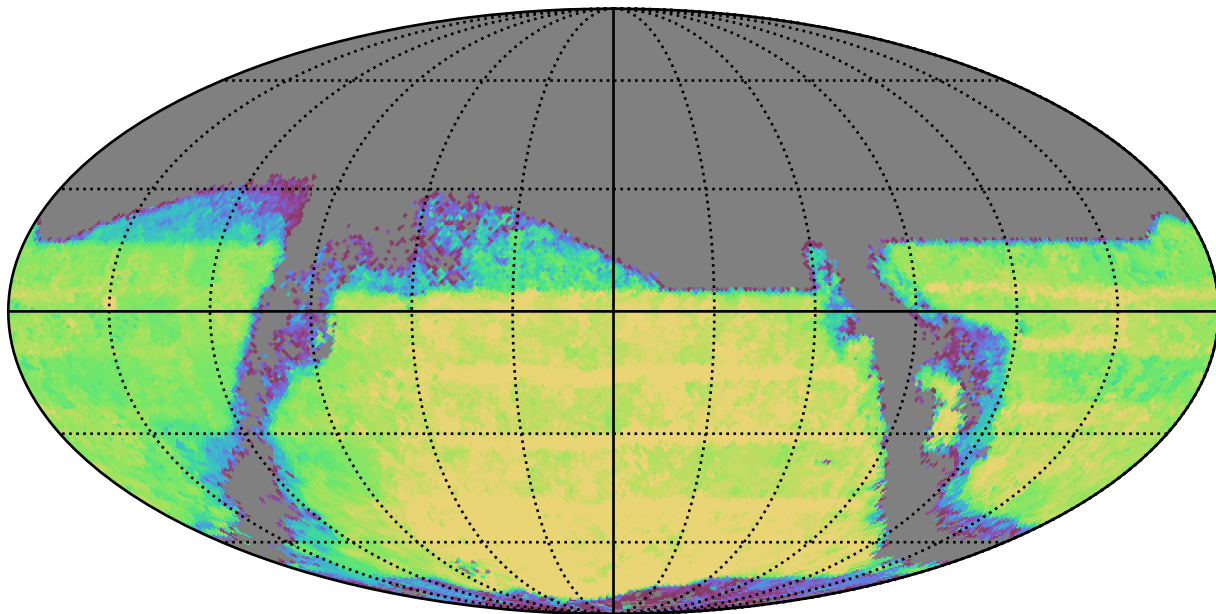
weather_cloudso1v3.4_10yrs : TDC_season
