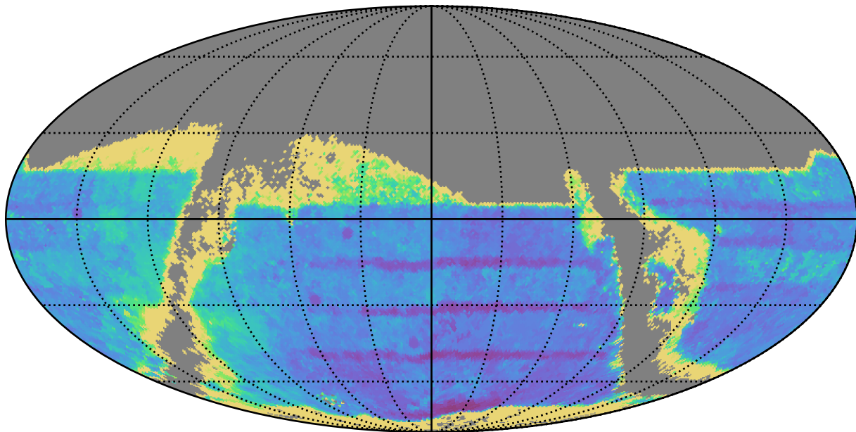
weather_cloudso1v3.4_10yrs : TDC_accuracy
