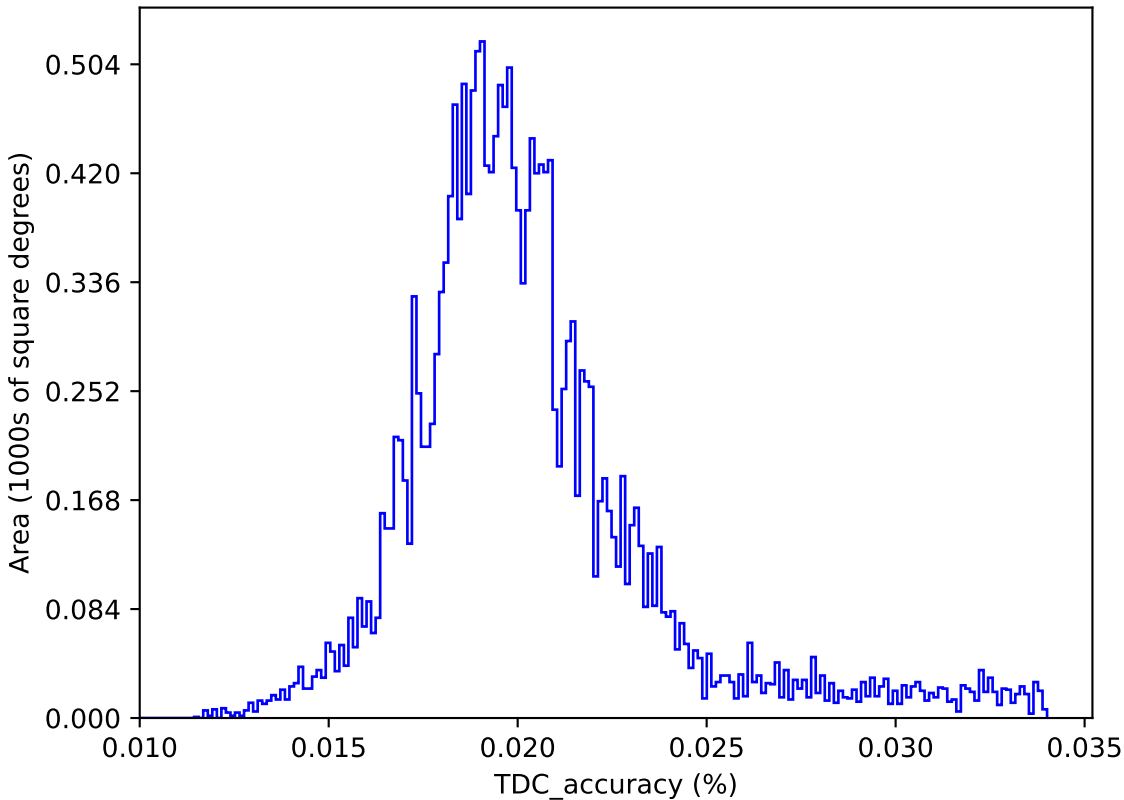
weather_cloudso1v3.4_10yrs : TDC_accuracy
